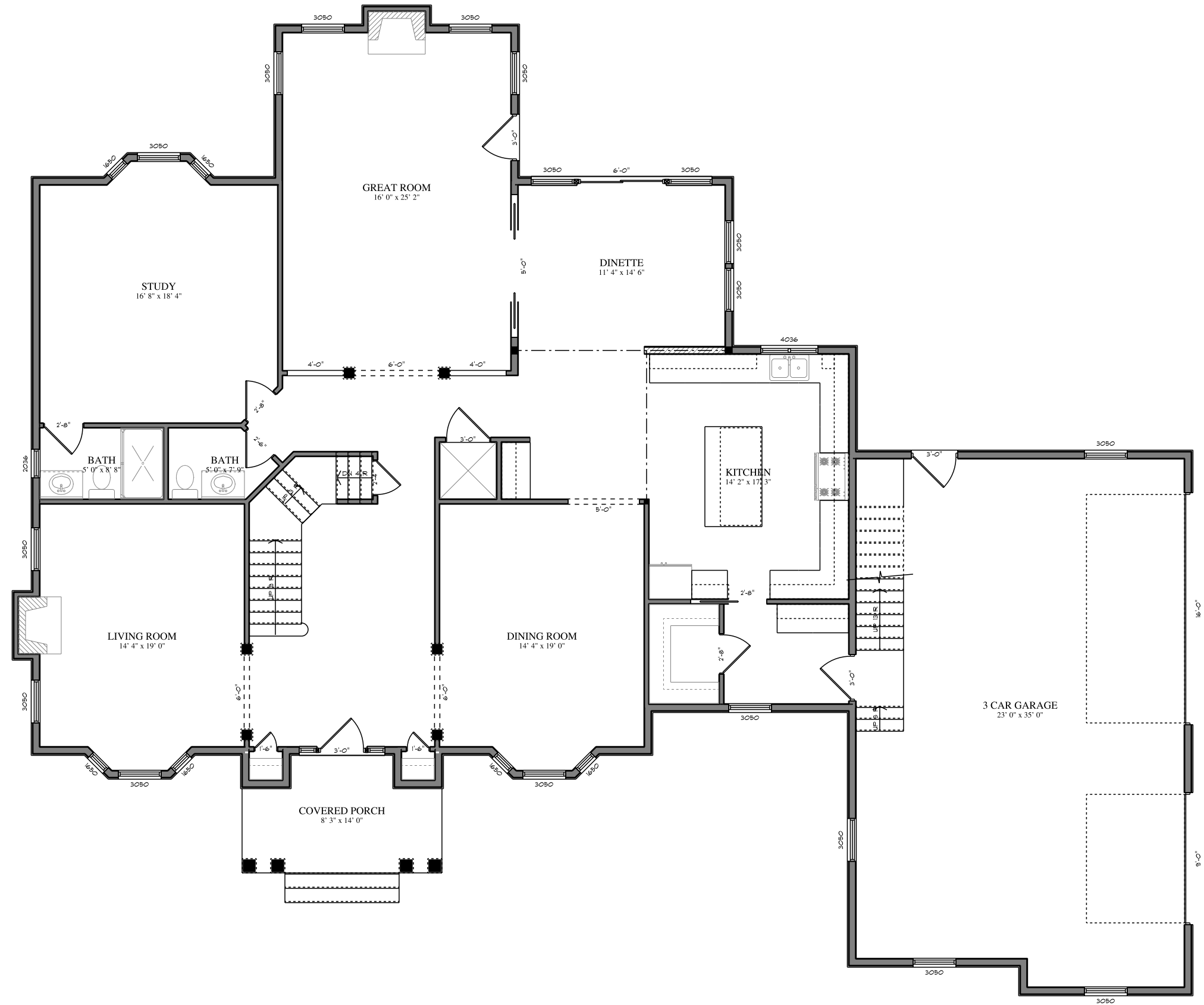
FIRST FLOOR PLAN 1/8" = 1'-0"
