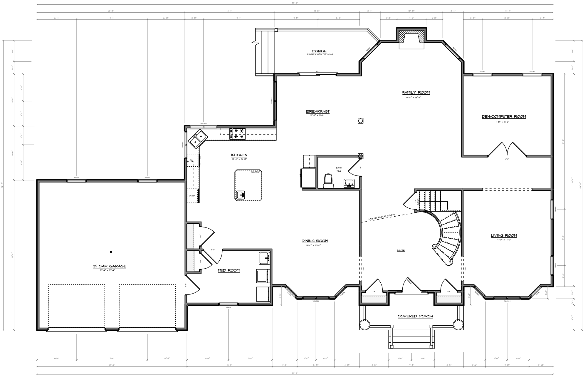
FIRST FLOOR PLAN SCALE: 1/4" = 1'-0"
